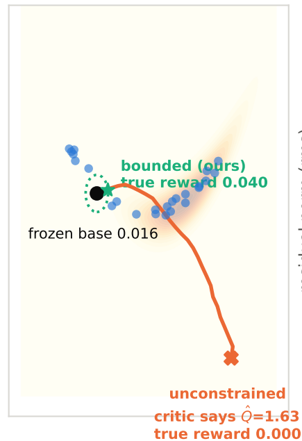
(c) same critic, two updates both follow \nabla_a Q ; only one keeps the policy where the critic is valid
