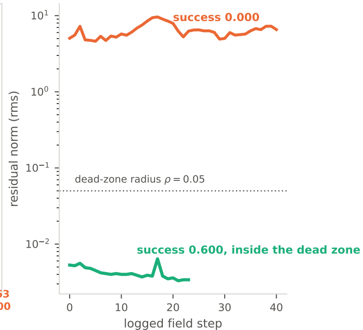
(d) measured on the red-mug task logged residual norm during real training (log scale)
