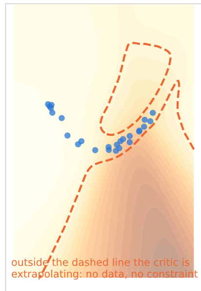
(b) what the critic believes learned Q ; dashed line = where it stops matching reality
