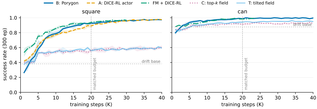
Figure 3: robomimic learning curves (300-episode evaluations every 1K steps; mean and min-max band over seeds; dashed vertical line marks the matched 20K budget). On square, Porygon overtakes the backpropagated control A by 7K steps and holds a 4–7-point lead through the matched budget; the value-only fields C/T flatline near 0.55. On can, Porygon and the flow-matching pipeline both approach the ceiling ( \geq 0.98 ). [TODO: regenerate with the s44 and can-baseline reruns when they finish.]
