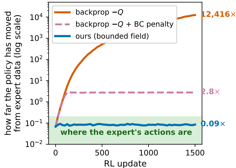
(b) why: the update size is set by the critic, so the policy escapes
