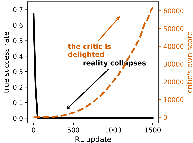
(a) backpropagating a critic: it optimises the score, not the task
