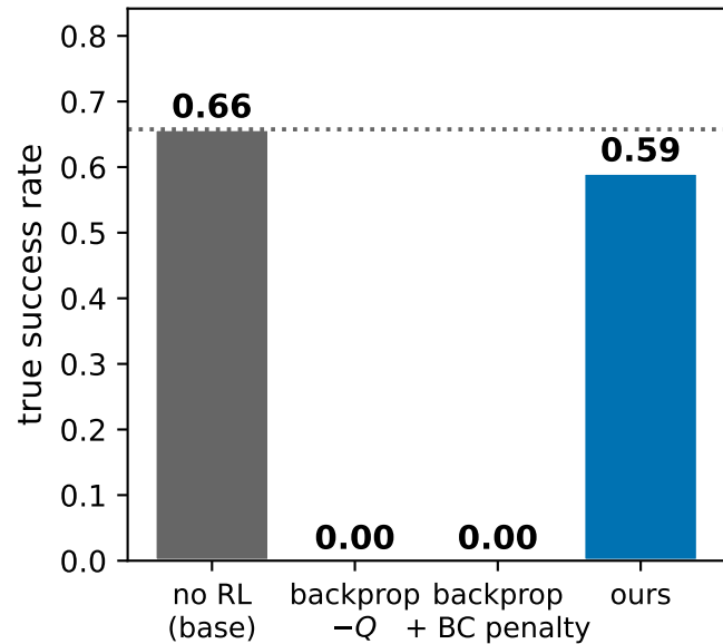
(c) the outcome: a penalty does not rescue it, a bounded step does
