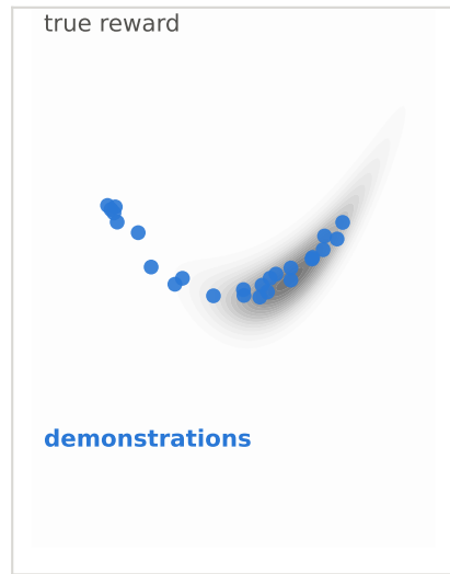
policy cloned from 25 demos; the critic sees only these (blue), all on the band (a) post-training starts here
