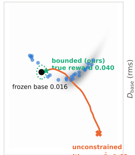
both follow \nabla_a \hat{Q} ; only one keeps the policy where the critic is valid (c) same critic, two updates
