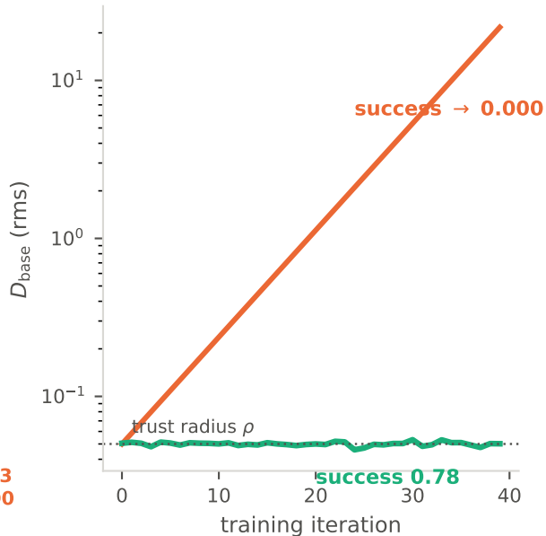
distance from the frozen base during led training (log scale) (d) measured on LIBERO t65
