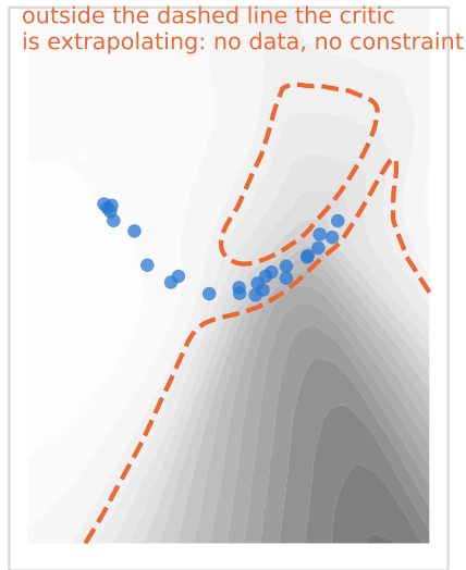
learned \hat{Q} ; dashed line = where it stops matching reality (b) what the critic believes
