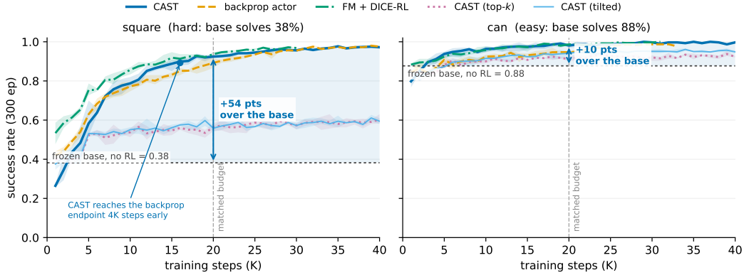
Figure 4: What post-training adds, and how fast. 300-episode evaluations every 1K steps; line is the seed mean, band the min-max over seeds. The dashed horizontal line is the frozen base — everything above it is what fine-tuning bought, shaded for CAST. On square, the discriminative task, CAST adds 54 points over the base at the matched 20K budget and reaches the backprop actor’s 20K endpoint about 4K steps earlier; the two resolution variants (top- k , tilted) stall near 0.55 and are analysed in Section 5.6. On can both updates approach the ceiling, so the task mainly checks that nothing breaks. Note that FM + DICE-RL runs on a different (flow-matching) base and so is not a same-base comparison; the same-base contrast is CAST against the backprop actor.
