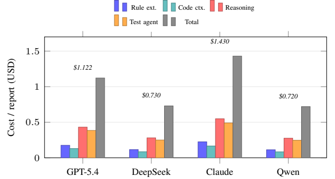
Fig. 2. Average model cost per submitted report by model family and pipeline stage. The GPT-5.4 bars correspond to Table VII
