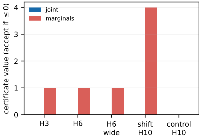
Same transcript, different retained information
