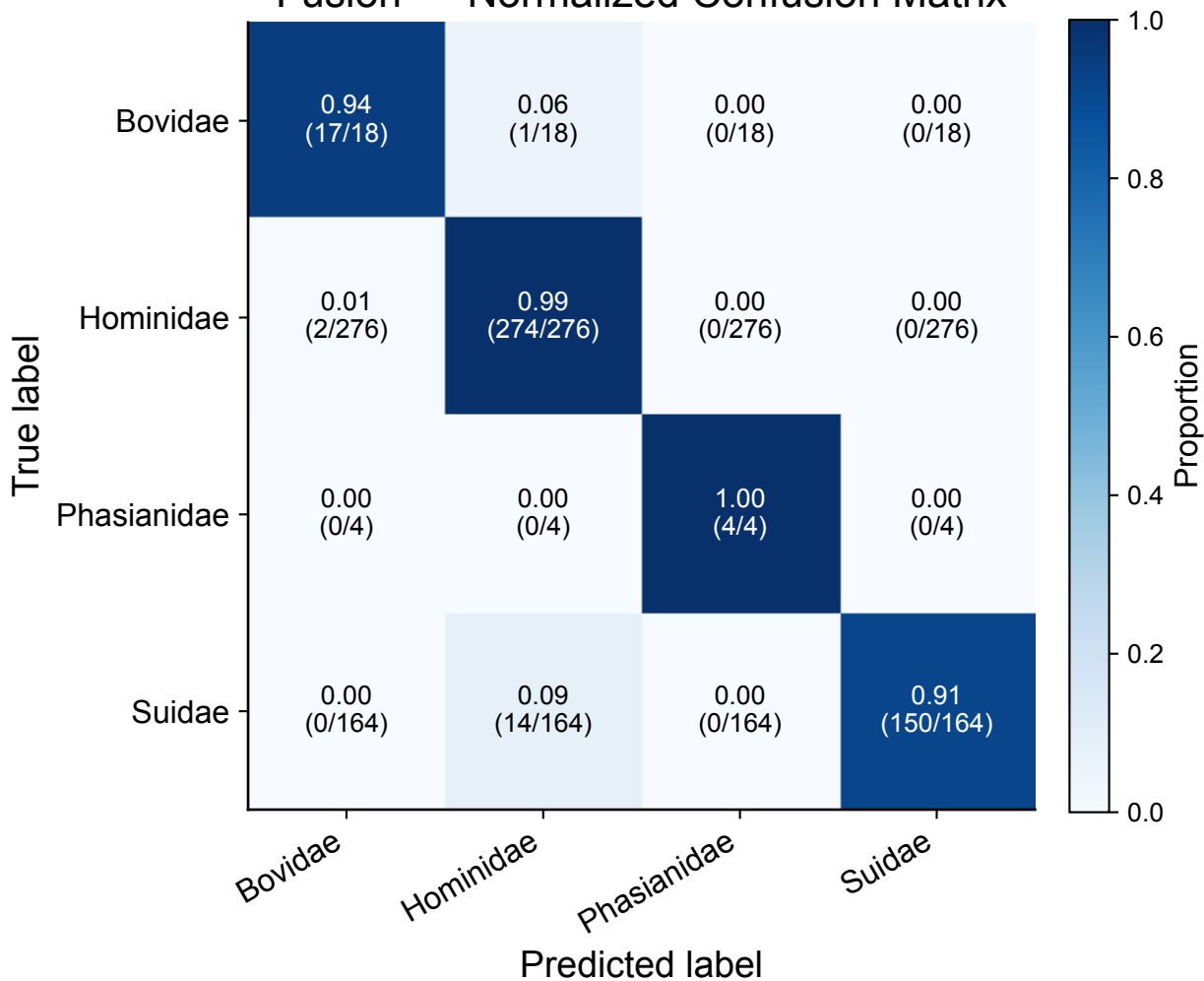
Fusion — Normalized Confusion Matrix
