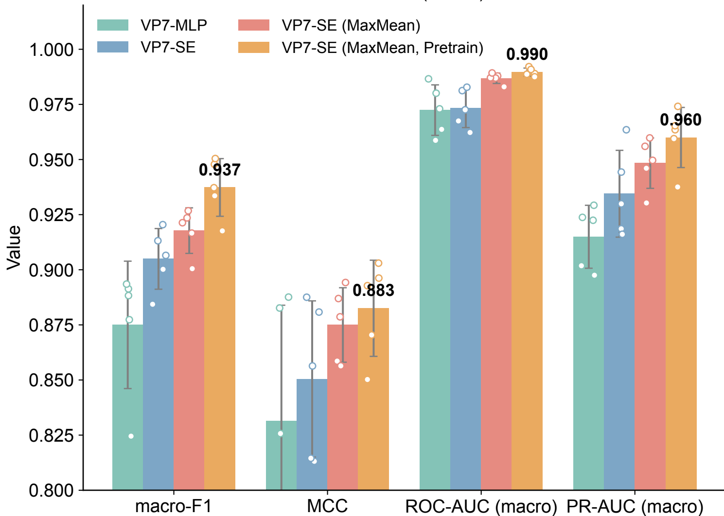
VP7 Models(5-Fold)
