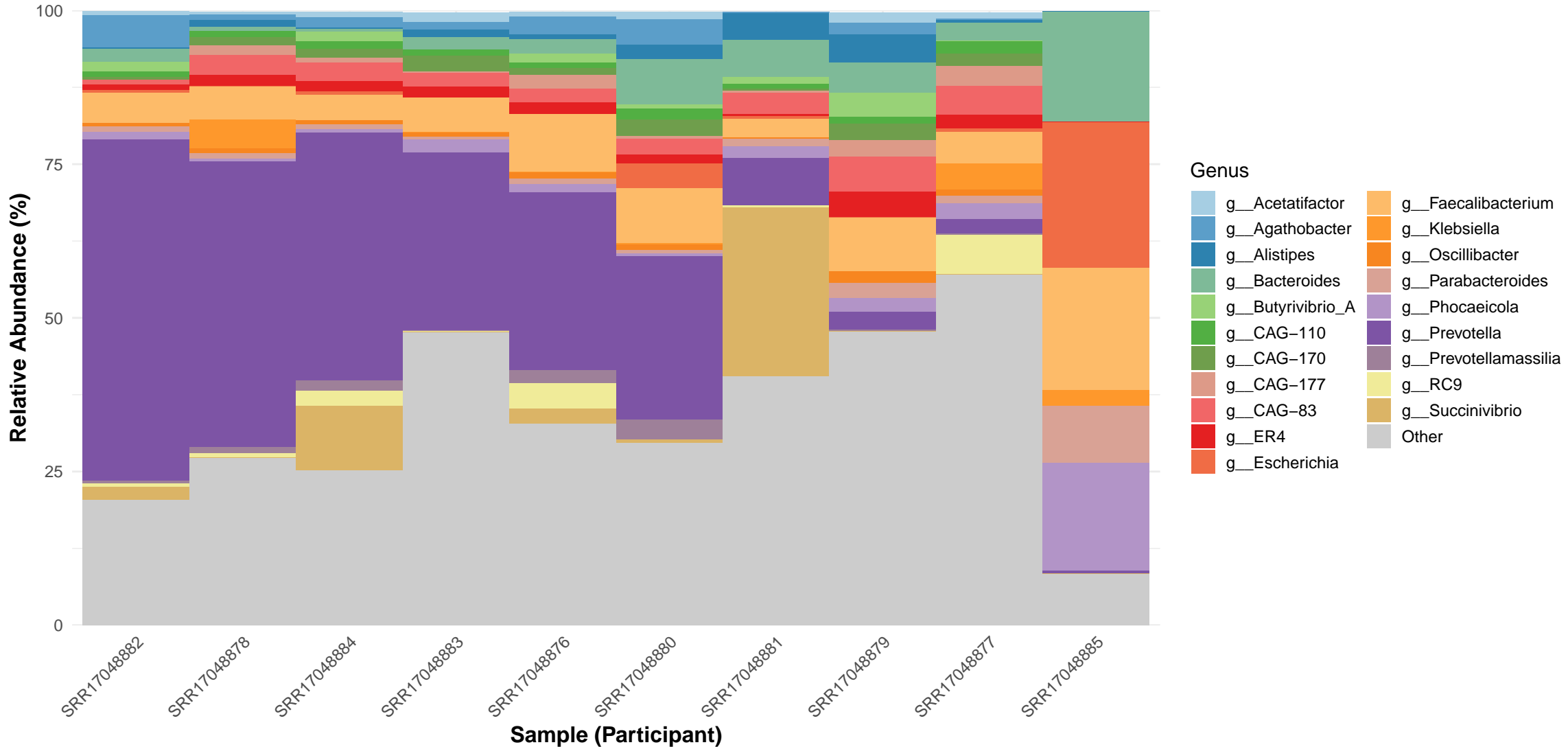
Gut Microbiome Composition at Genus Level
