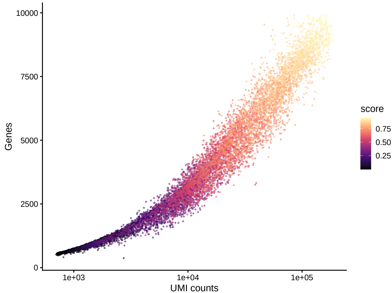
Doublet score (heuristic)
