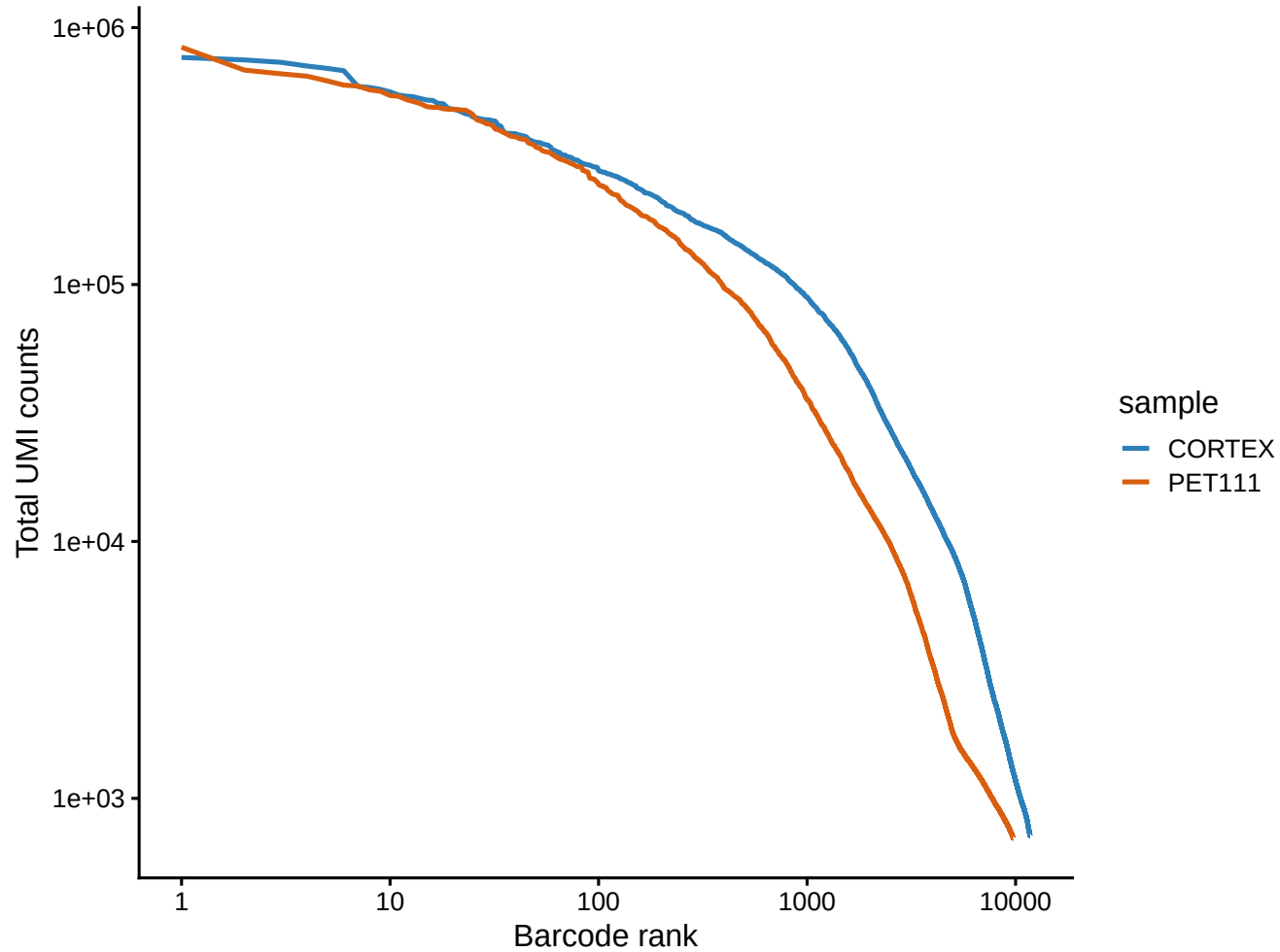
Barcode-rank (knee) plot
