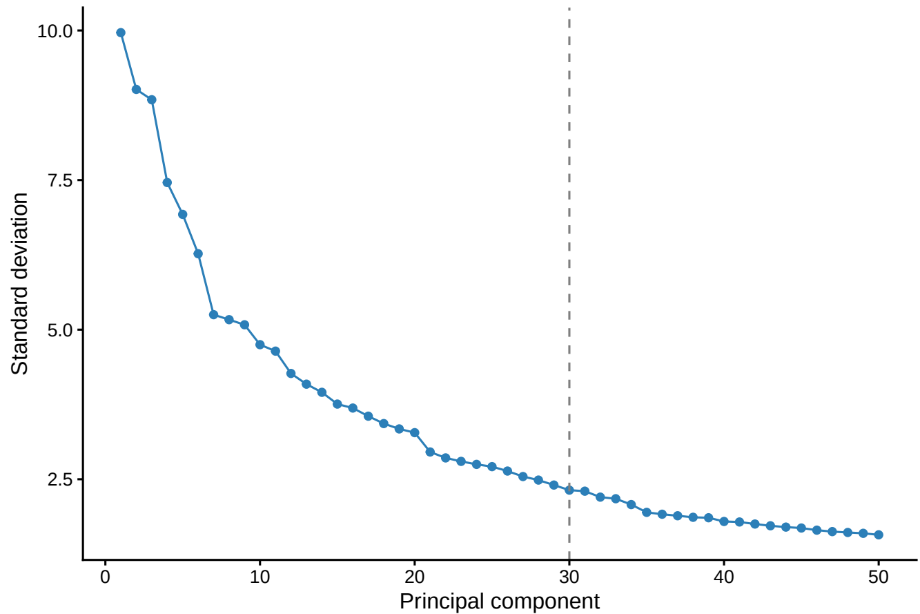
Elbow plot
