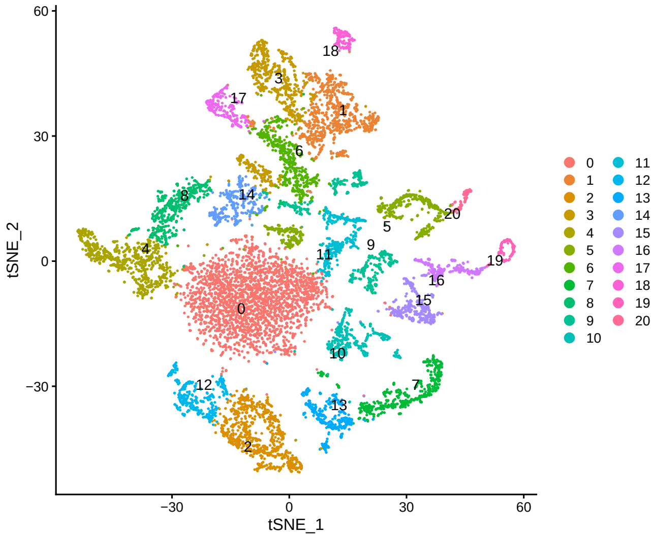
t-SNE (clusters)
