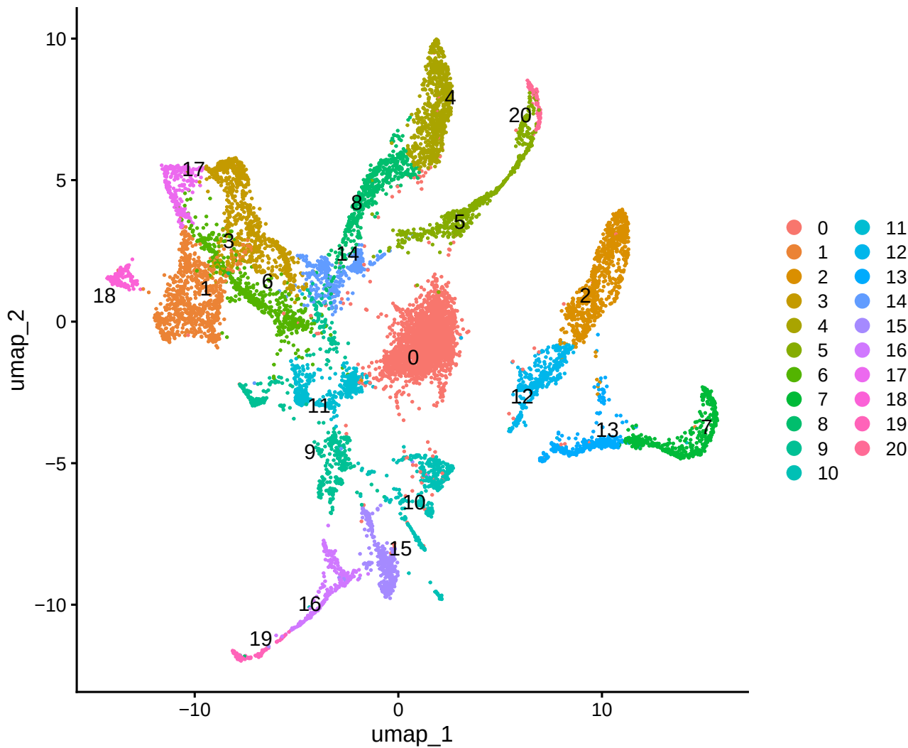
UMAP (clusters)
