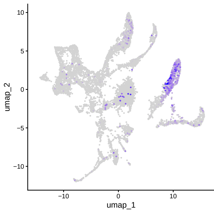
AT3G29410
