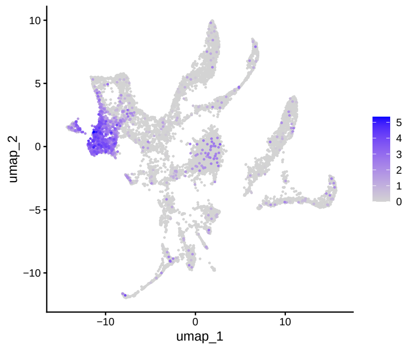
AT1G19250
