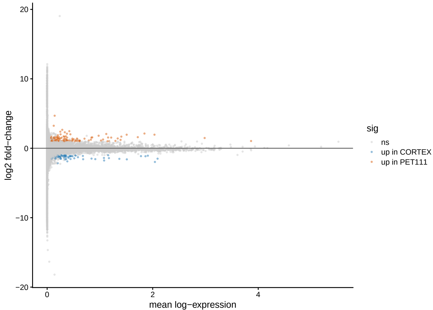
MA plot: PET111 vs CORTEX
