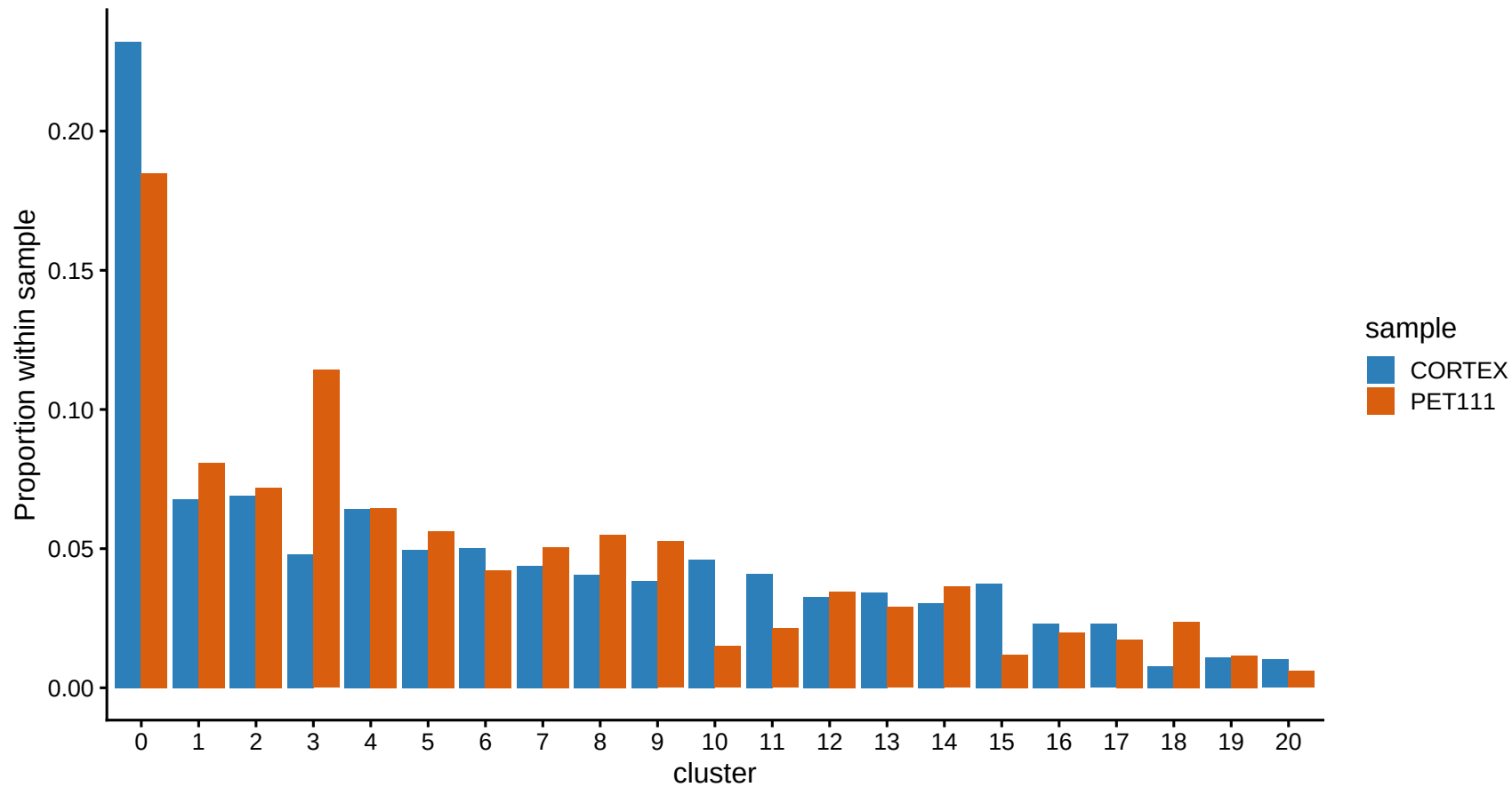
Per-cluster abundance: PET111 vs CORTEX
