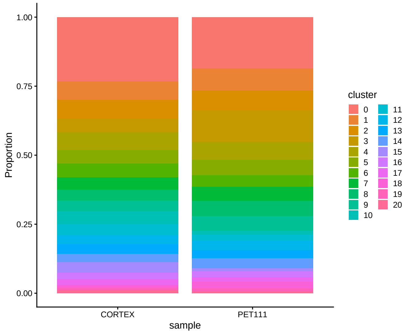
Cell-type composition per sample
