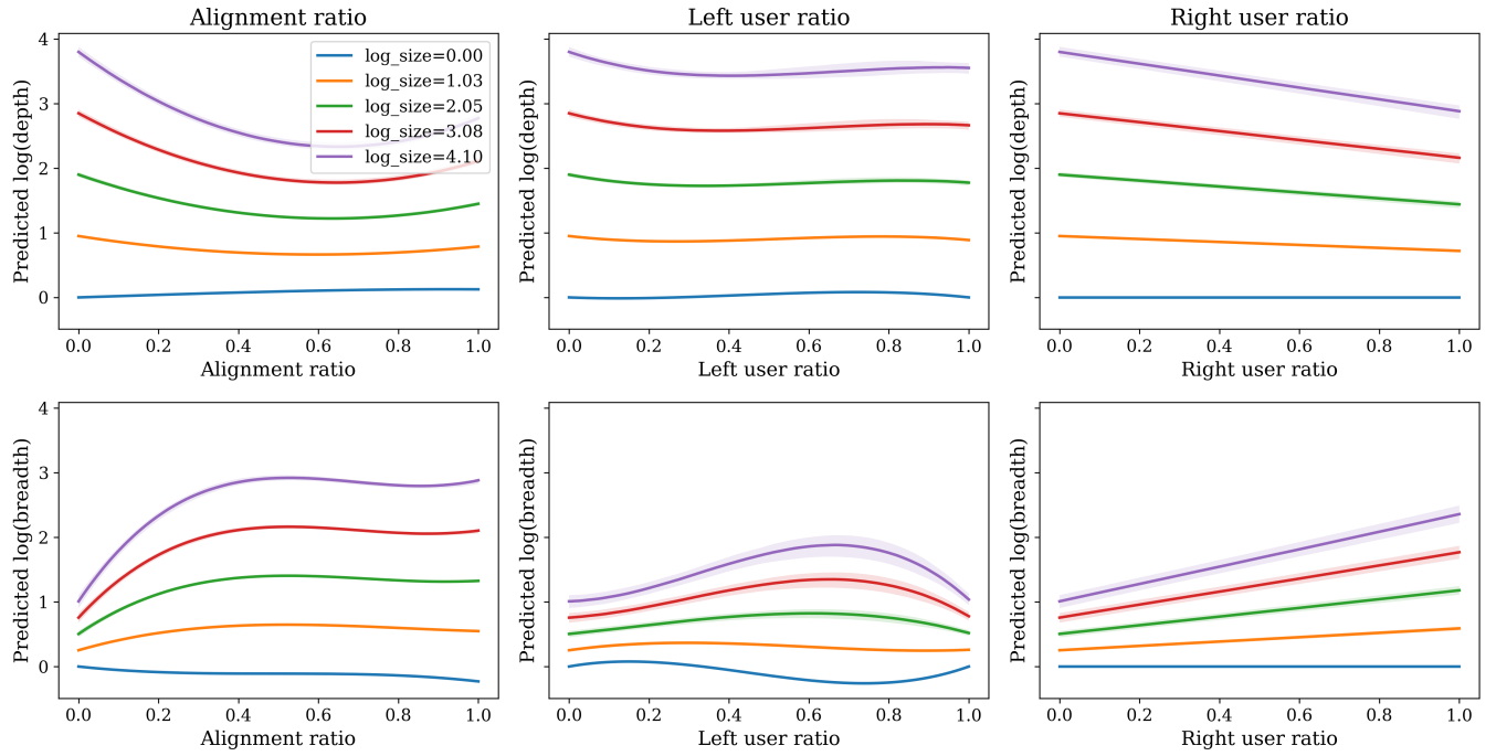
Figure 11: Marginal effects of ideological alignment, left-user ratio, and right-user ratio on cascade structure. Solid lines denote predicted log(depth) (top row) and log(breadth) (bottom row) at five equally spaced values of log(size). Shaded bands represent 95% bootstrap confidence intervals. Homogeneous cascades (high alignment) tend to flatten into wide, shallow structures; heterogeneous cascades deepen through sequential exchanges.
