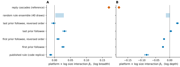
Figure A4: Platform-by-size interaction \beta_3 for repost cascades under alternative reconstruction rules (dots with 95% confidence intervals; shaded band, range over 40 random-rule draws), for log breadth (A) and log depth (B). The diamond marks the reply-cascade interaction under the same estimator.
