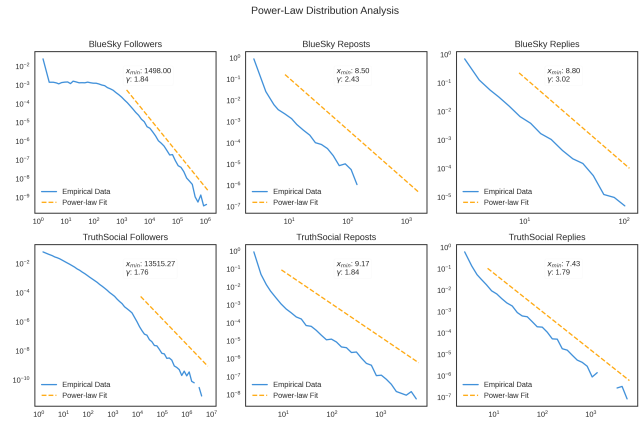
Figure 6: Follower count distributions across platforms.
