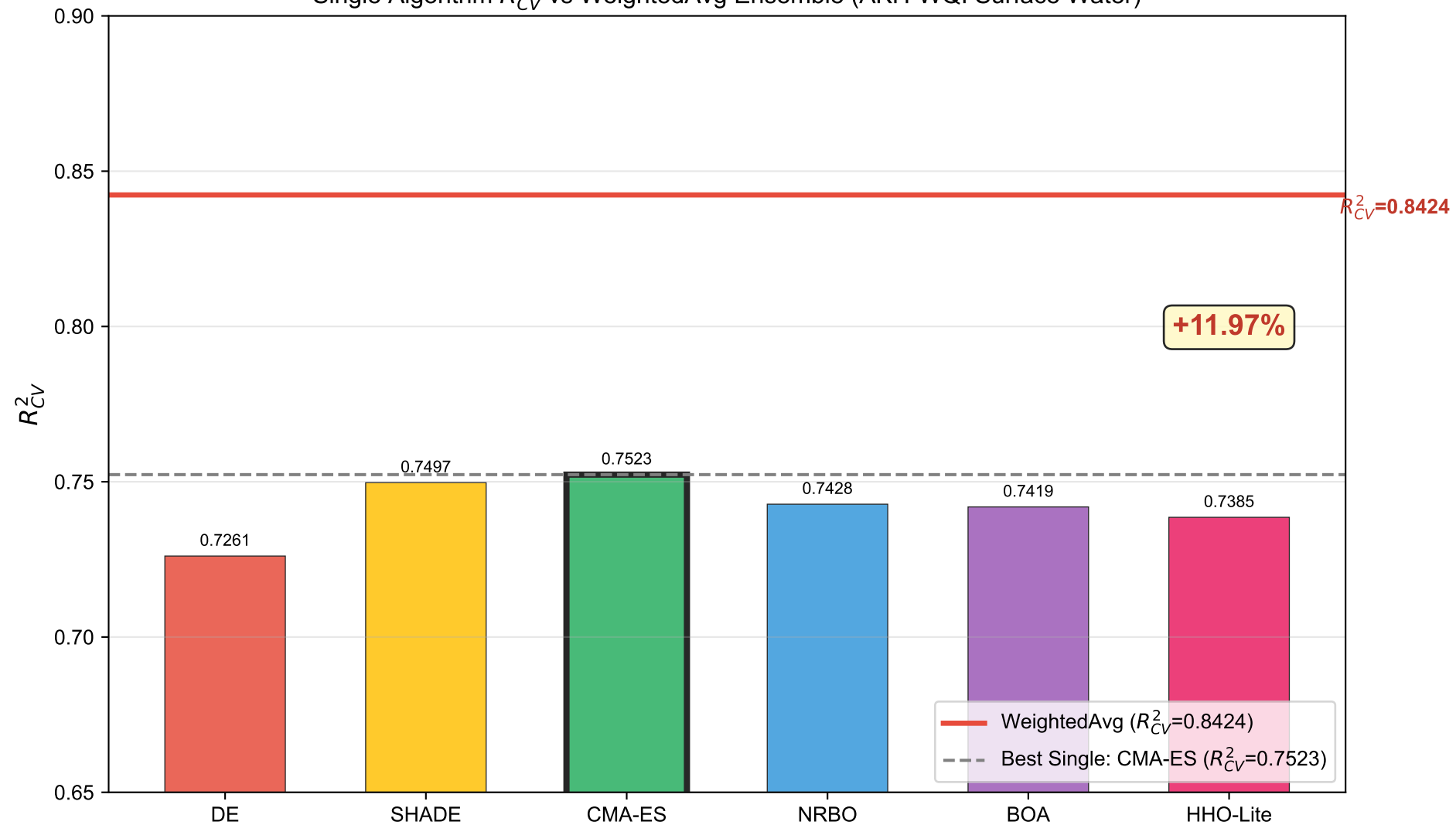
Single Algorithm R^2_{CV} vs WeightedAvg Ensemble (AKH-WQI Surface Water)
