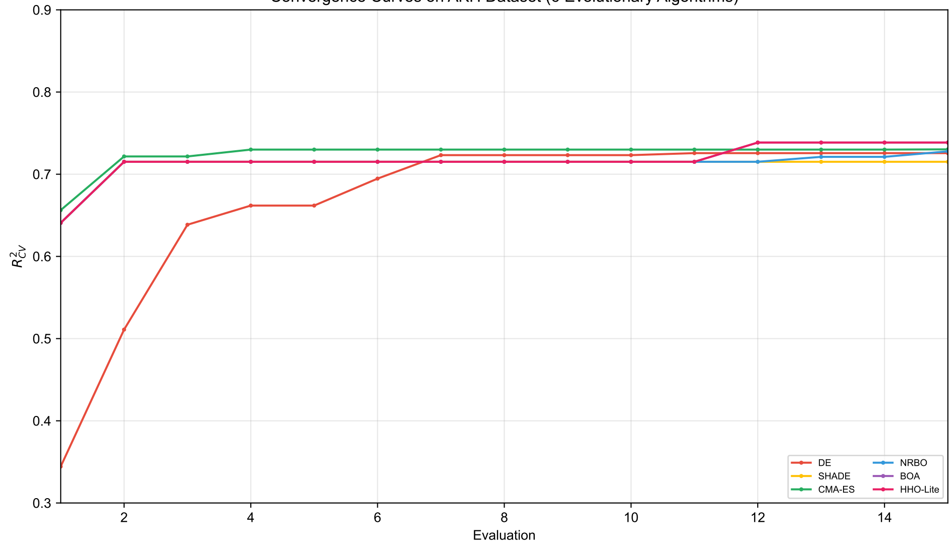
Convergence Curves on AKH Dataset (6 Evolutionary Algorithms)
