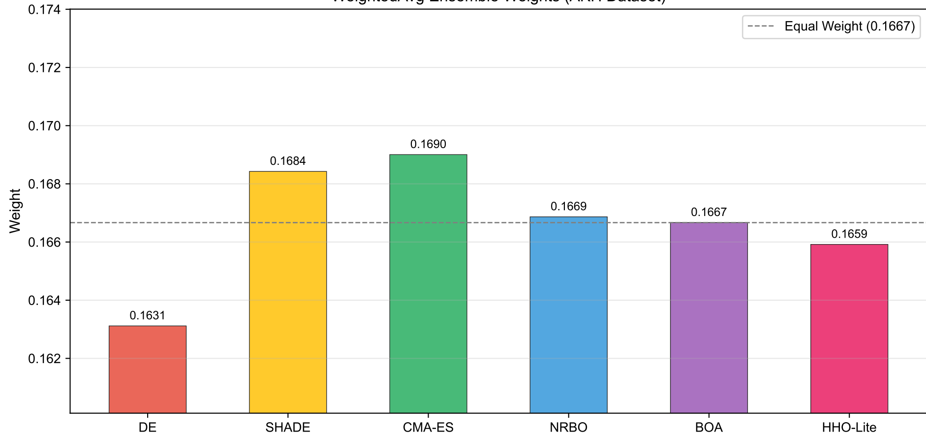
WeightedAvg Ensemble Weights (AKH Dataset)
