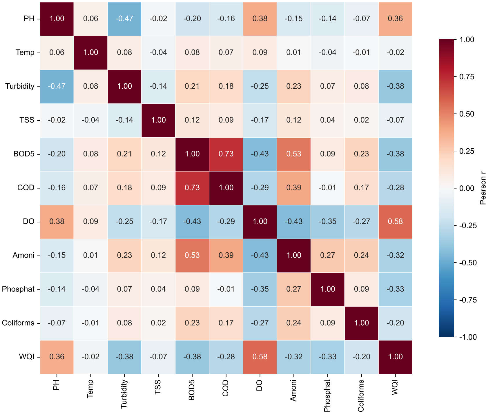
Feature Correlation Matrix (AKH-WQI, 10 Indicators + WQI)
