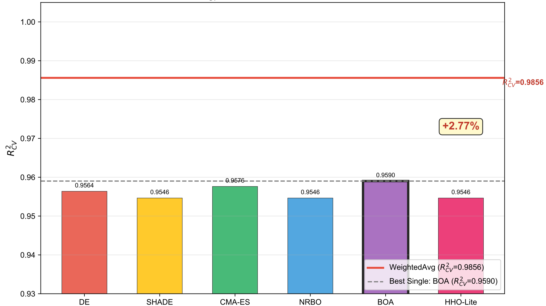
Single Algorithm R_{CV}^2 vs WeightedAvg Ensemble (Irish-River-CCME)
