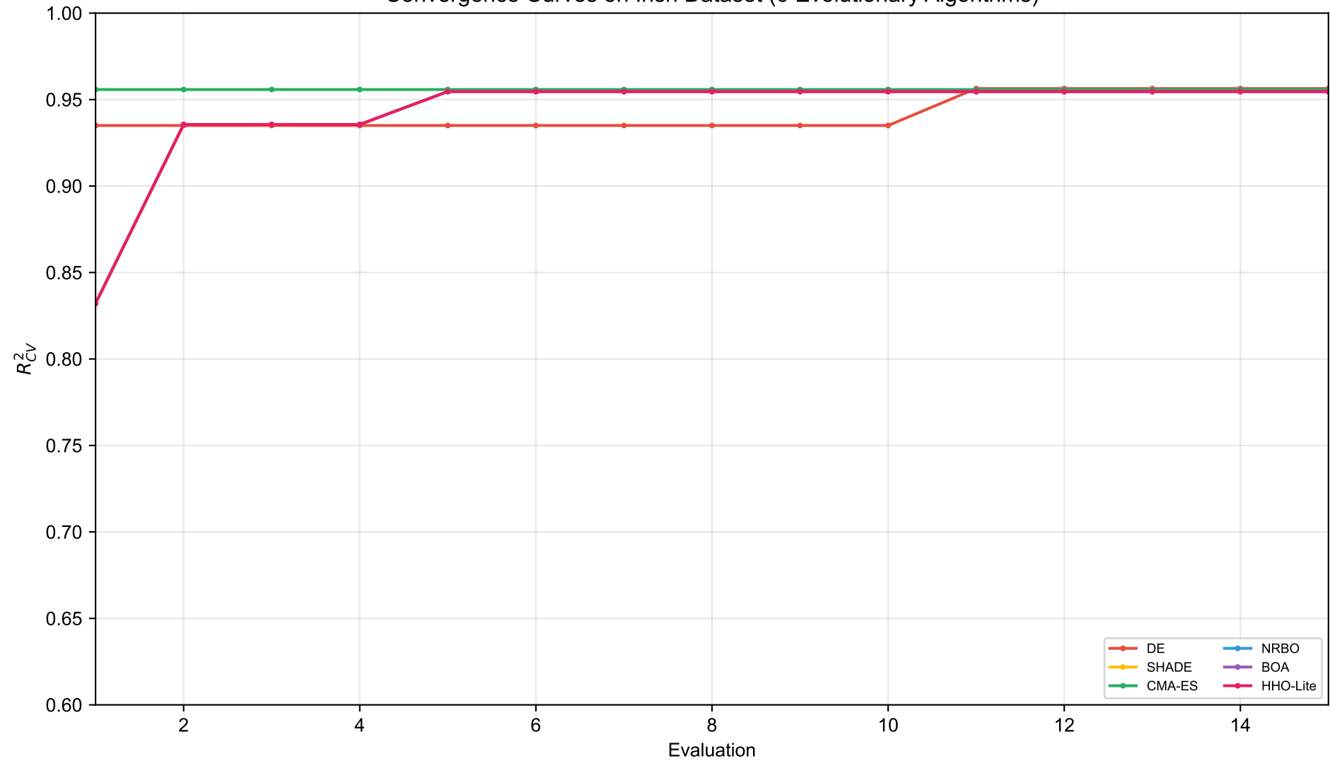
Convergence Curves on Irish Dataset (6 Evolutionary Algorithms)
