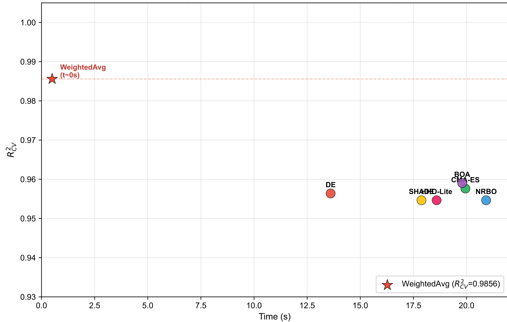
Accuracy vs Computational Efficiency (Irish-River-CCME)
