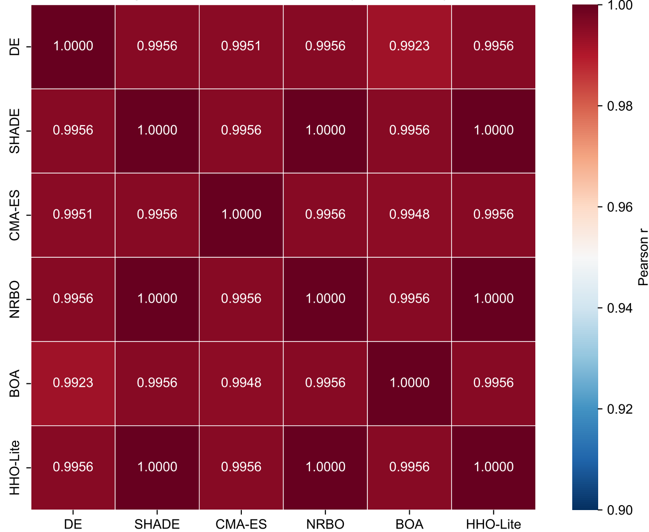
Algorithm Prediction Correlation (Irish Dataset)
