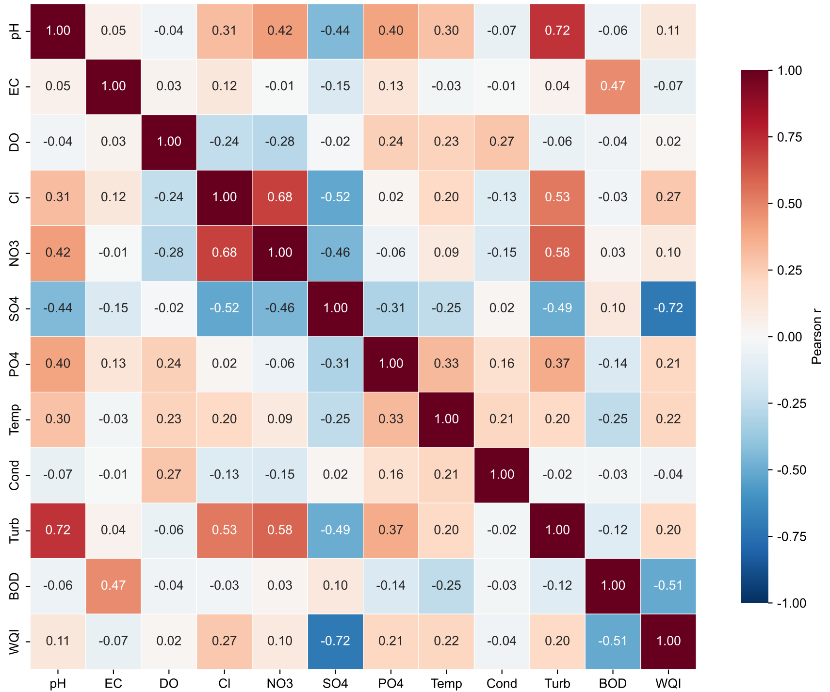
Feature Correlation Matrix (Irish-River-CCME, 11 Indicators + WQI)
