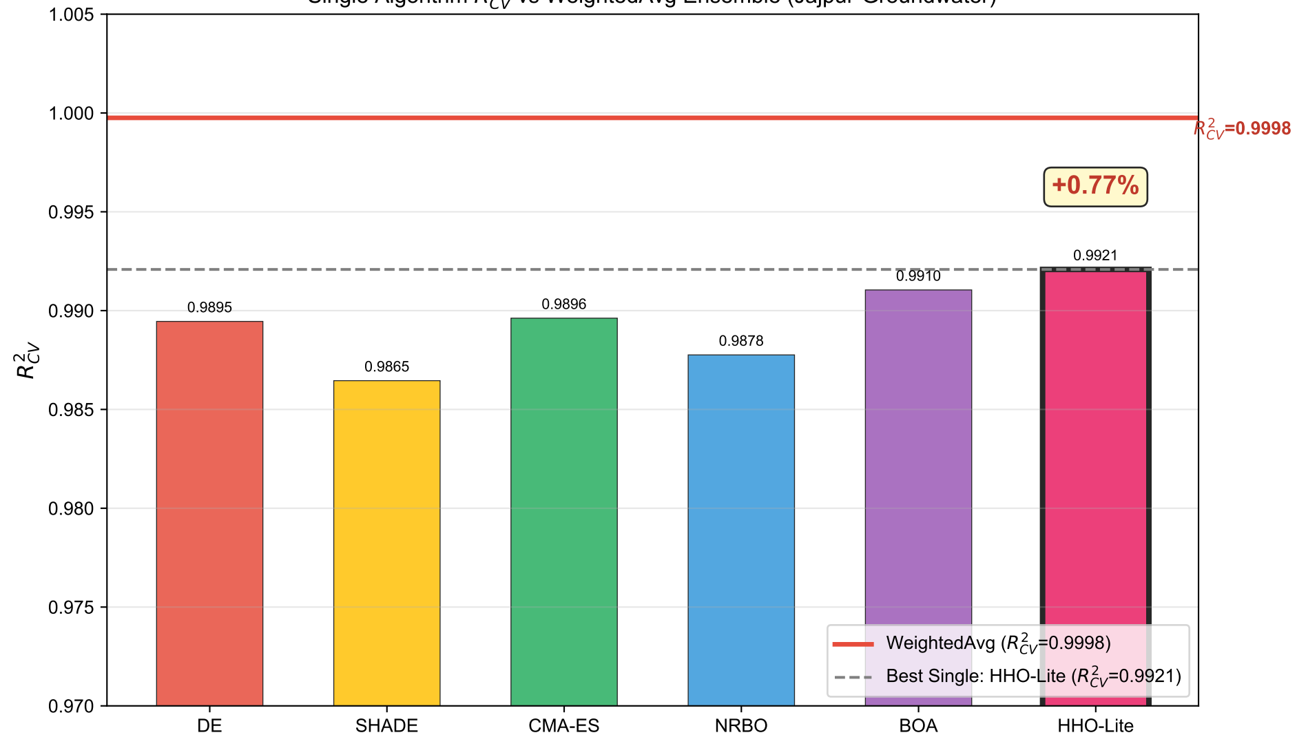
Single Algorithm R^2_{CV} vs WeightedAvg Ensemble (Jajpur-Groundwater)
