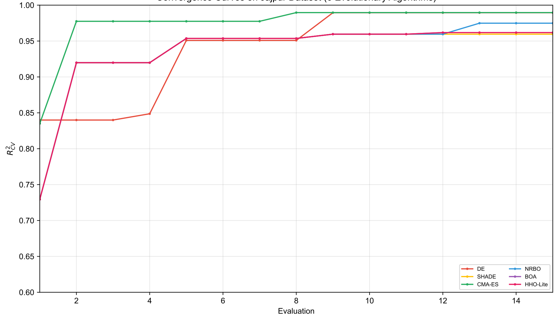
Convergence Curves on Jajpur Dataset (6 Evolutionary Algorithms)
