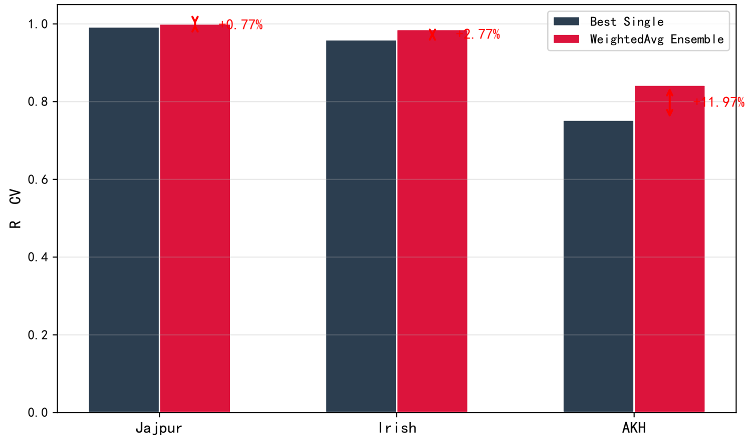
Ensemble Gain: Best Single vs WeightedAvg
