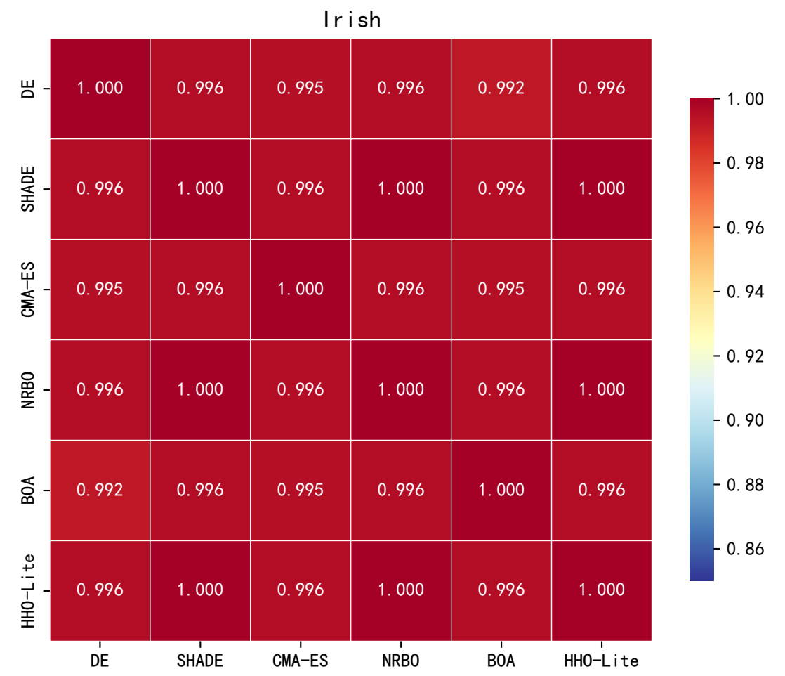
Prediction Correlation (Pearson r) Between Algorithms
