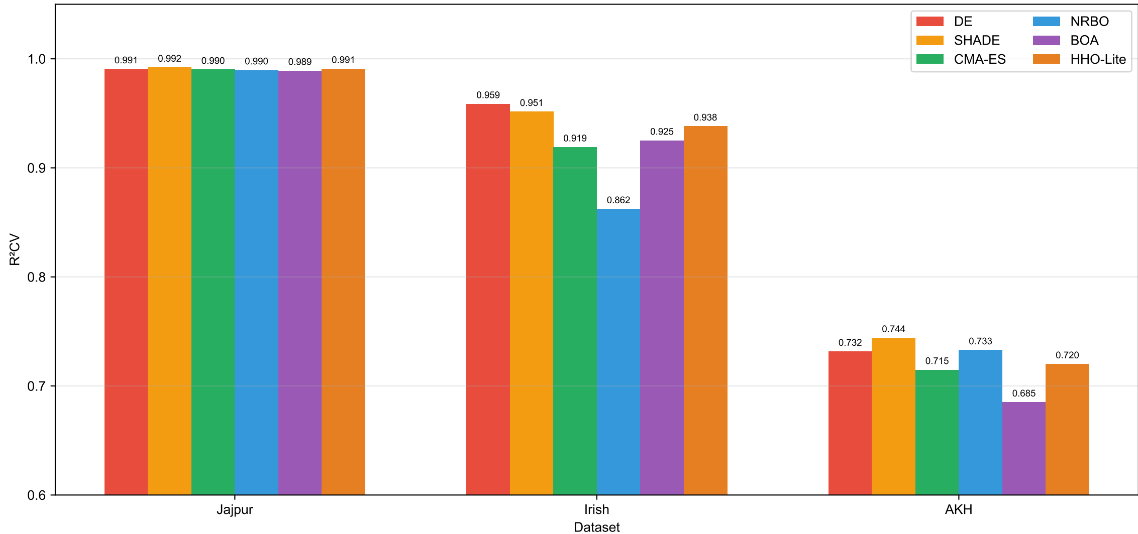
R 2 CV Comparison across Datasets (6 Evolutionary Algorithms)
