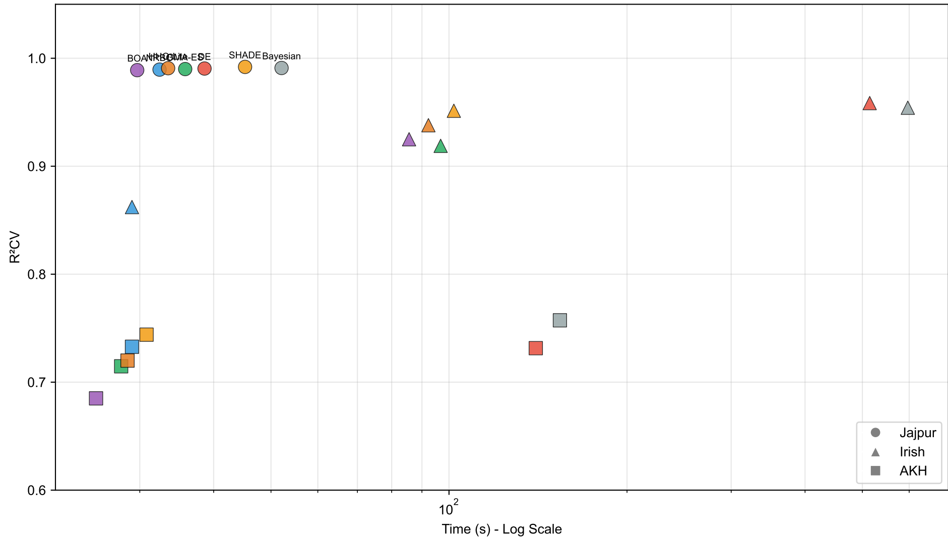
Pareto Chart: Accuracy vs Computational Efficiency
