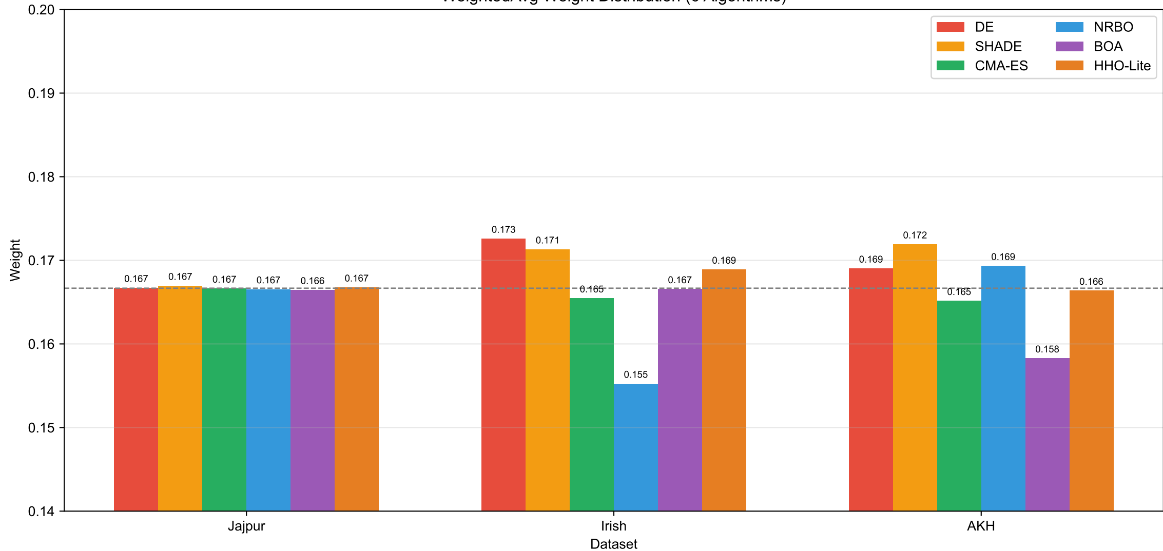
WeightedAvg Weight Distribution (6 Algorithms)
