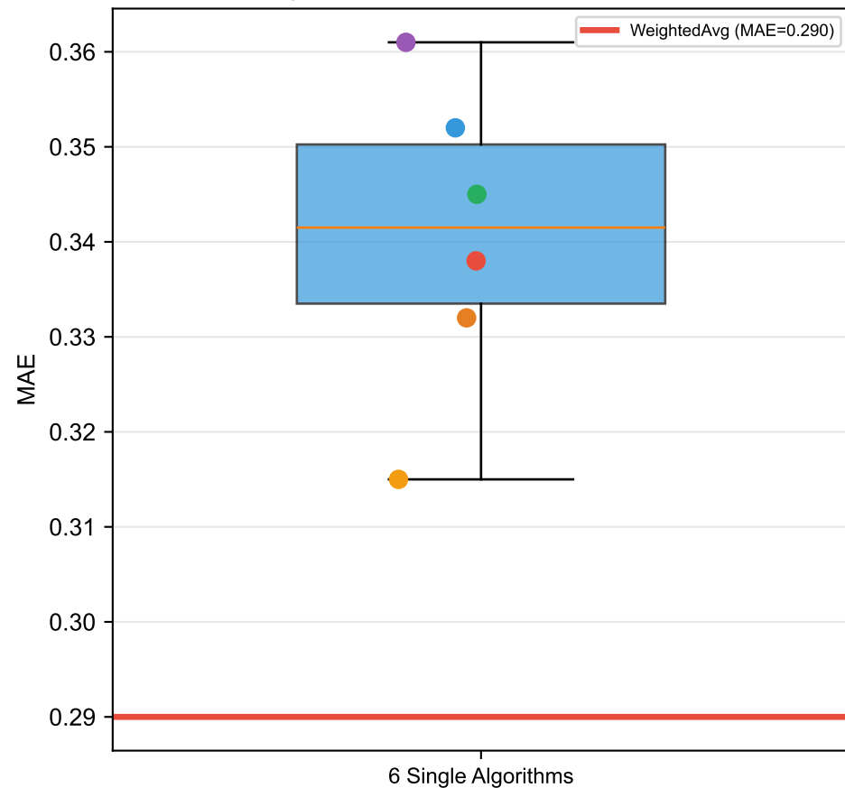
Jajpur Dataset - MAE Comparison
