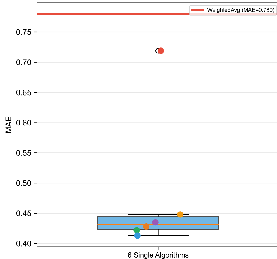
Irish Dataset - MAE Comparison
