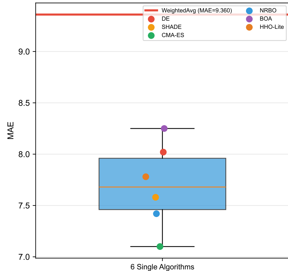
AKH Dataset - MAE Comparison
