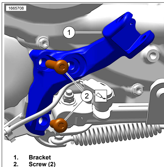
Figure 4. Left Side Footrest Bracket
