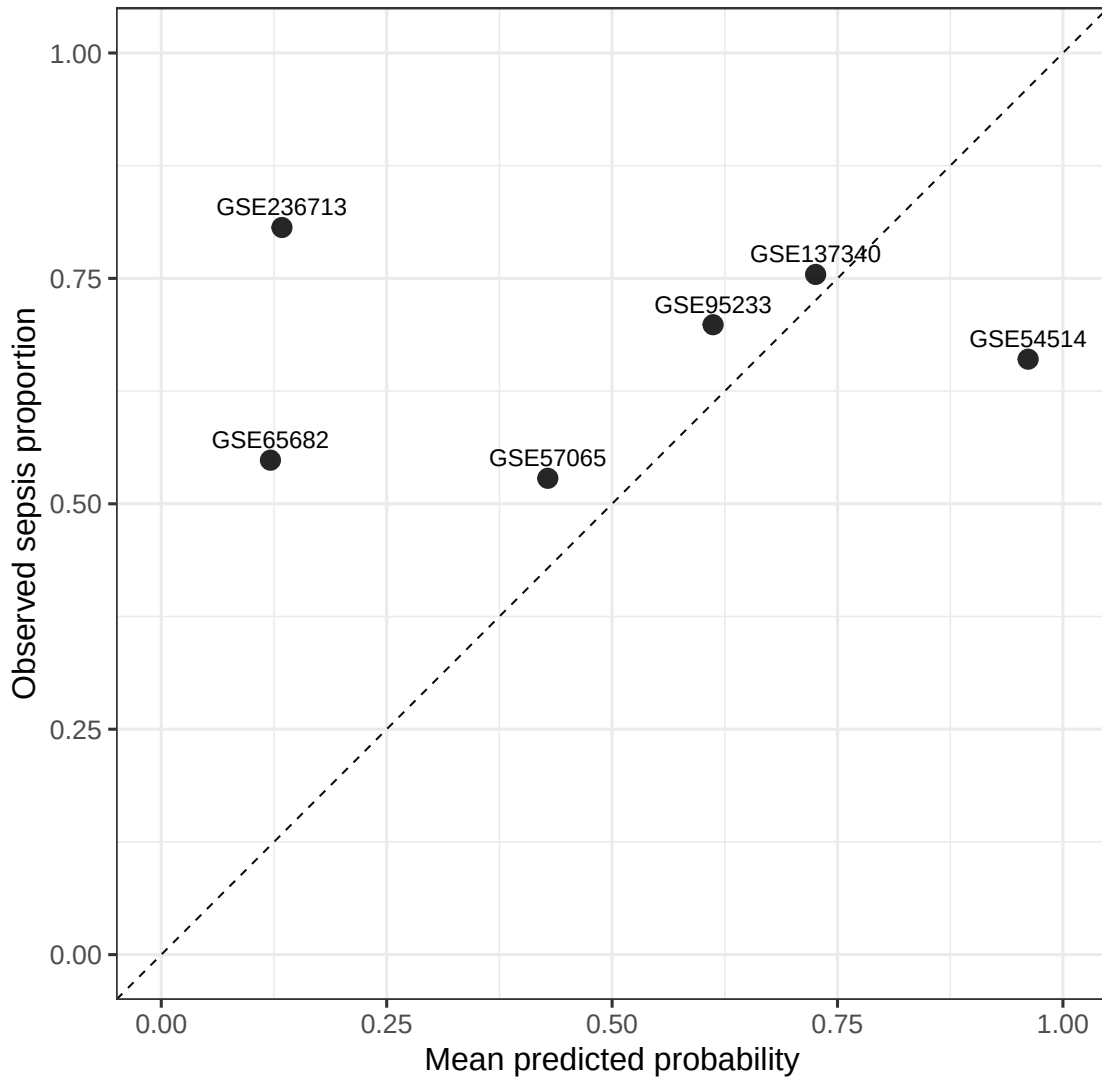
Observed rate vs mean predicted probability
