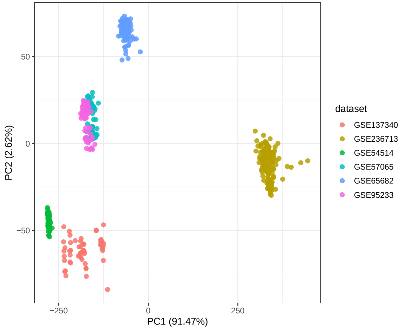
PCA of unadjusted expression by dataset
