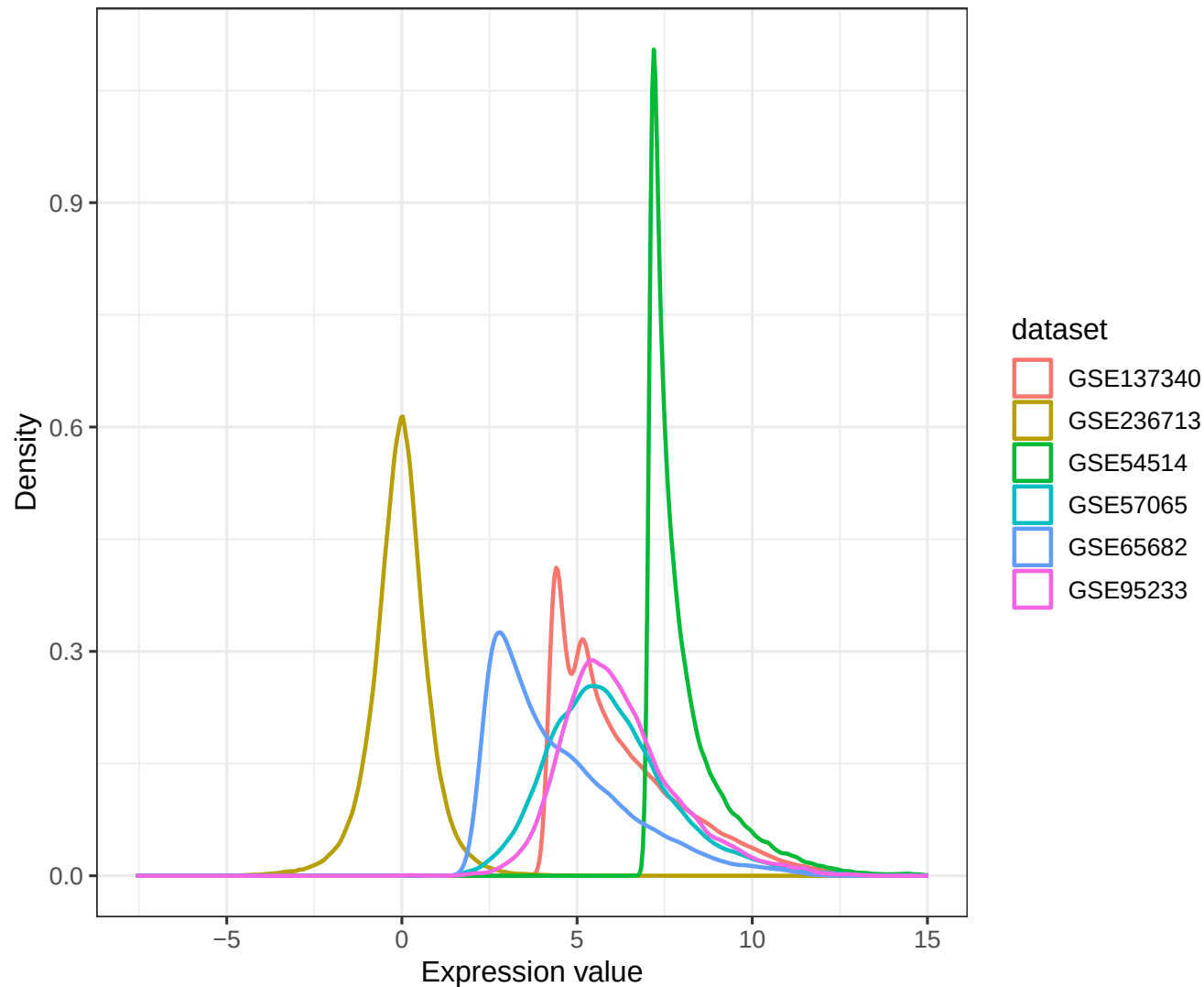
Expression density before batch visualization adjustment
