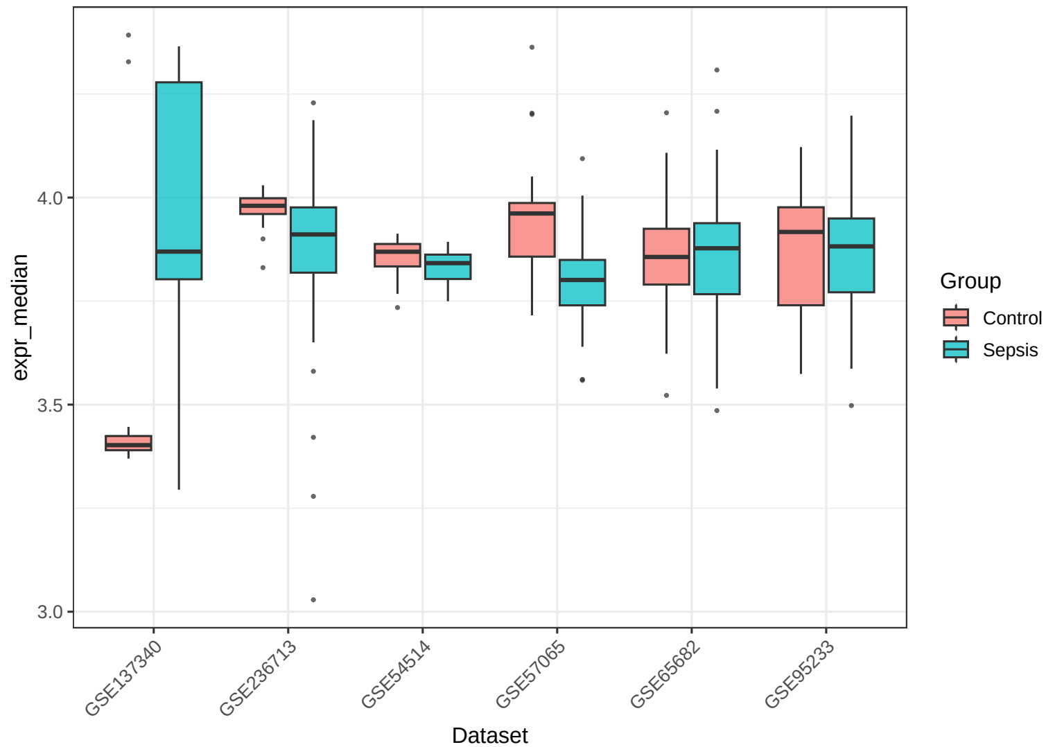
Sample median expression after ComBat adjustment
