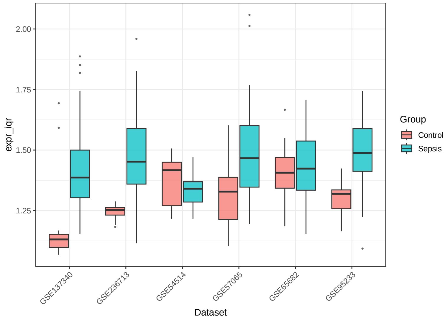
Sample expression IQR after ComBat adjustment
