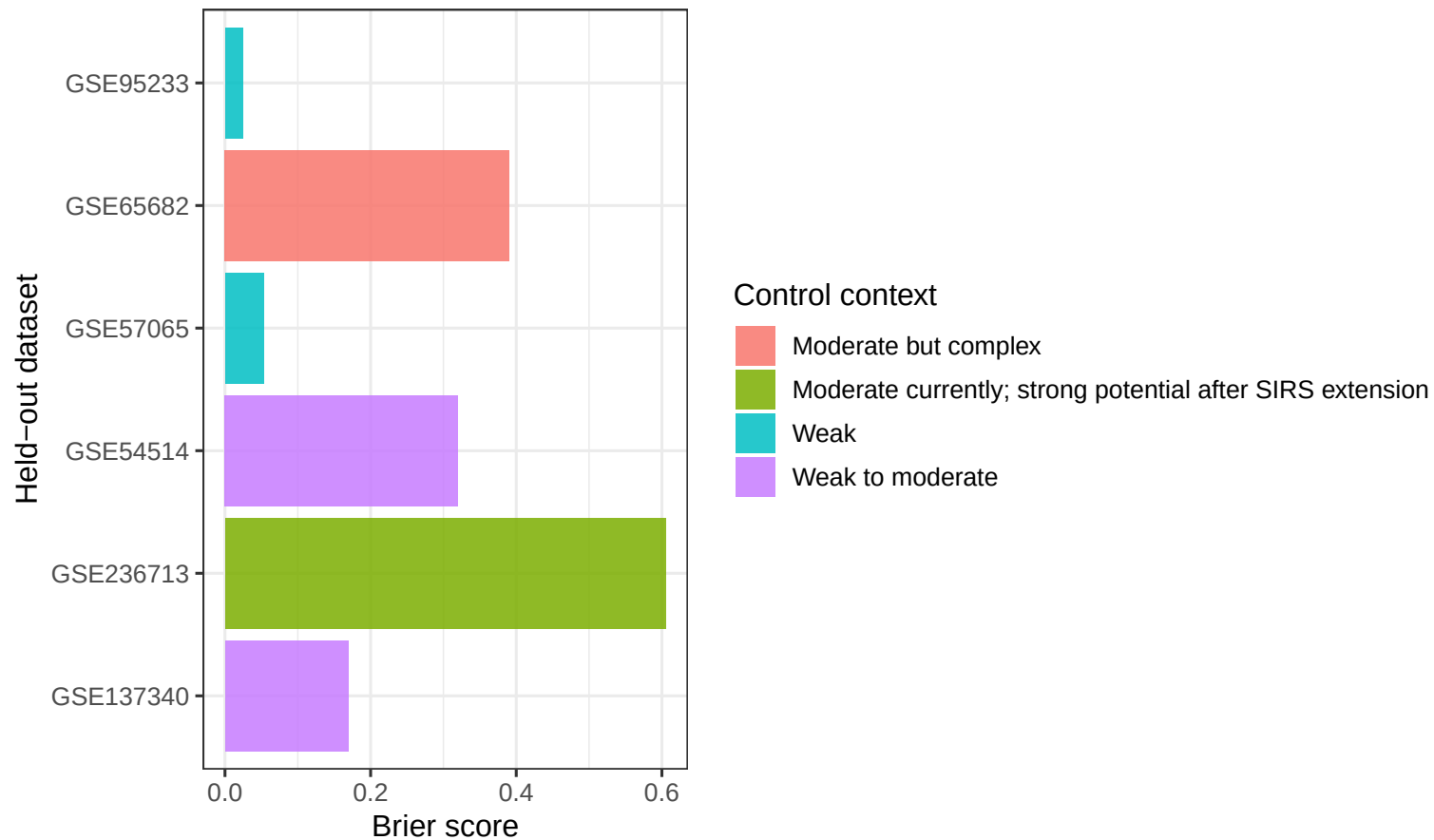
Nested LODO Brier score by cohort
