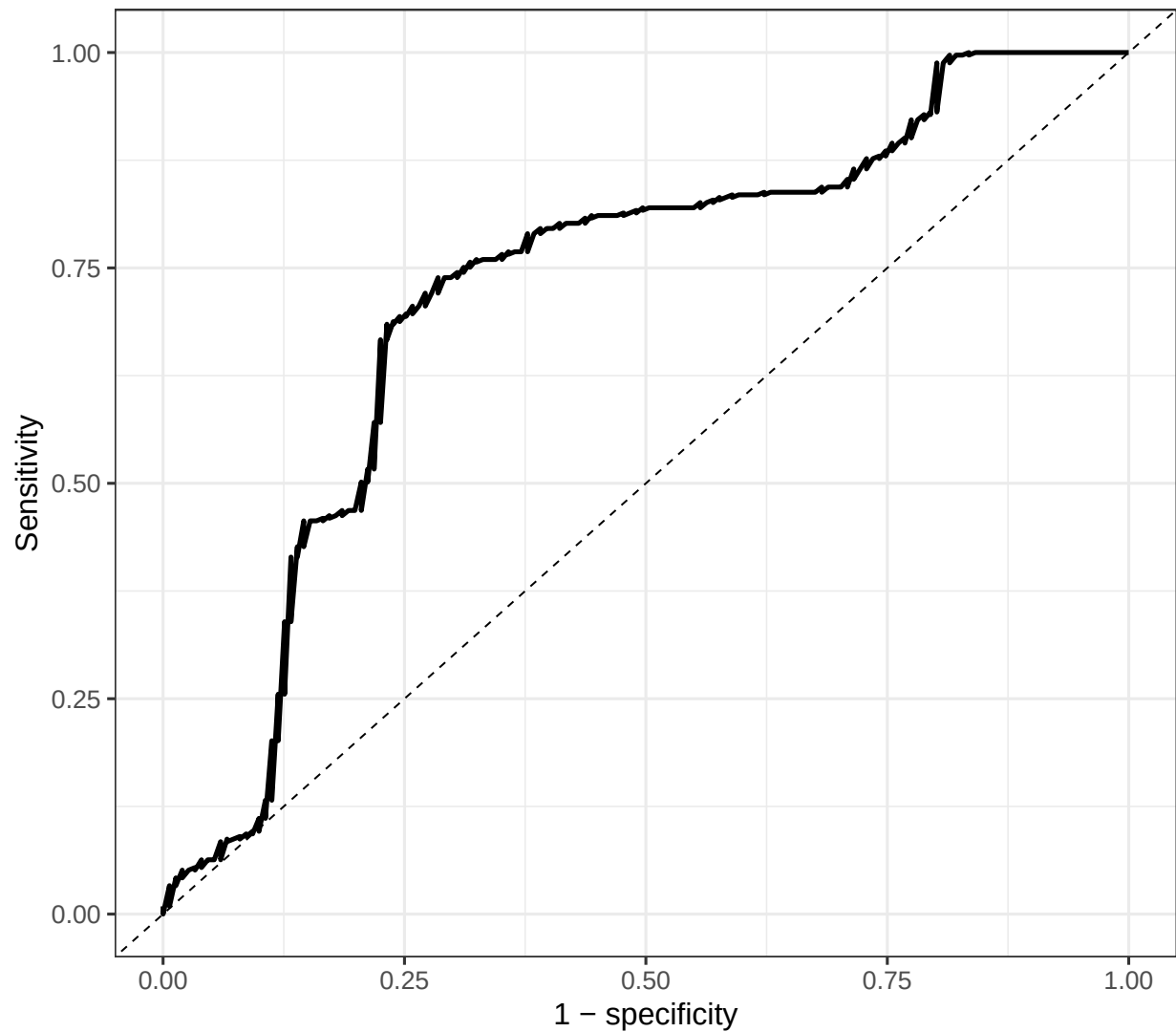
Pooled nested LODO ROC, AUROC = 0.722
