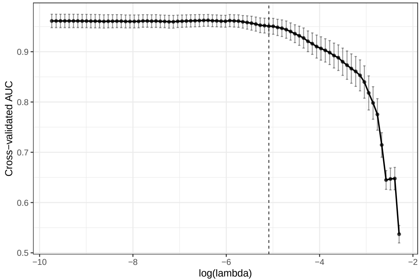
Final model cross-validation curve
