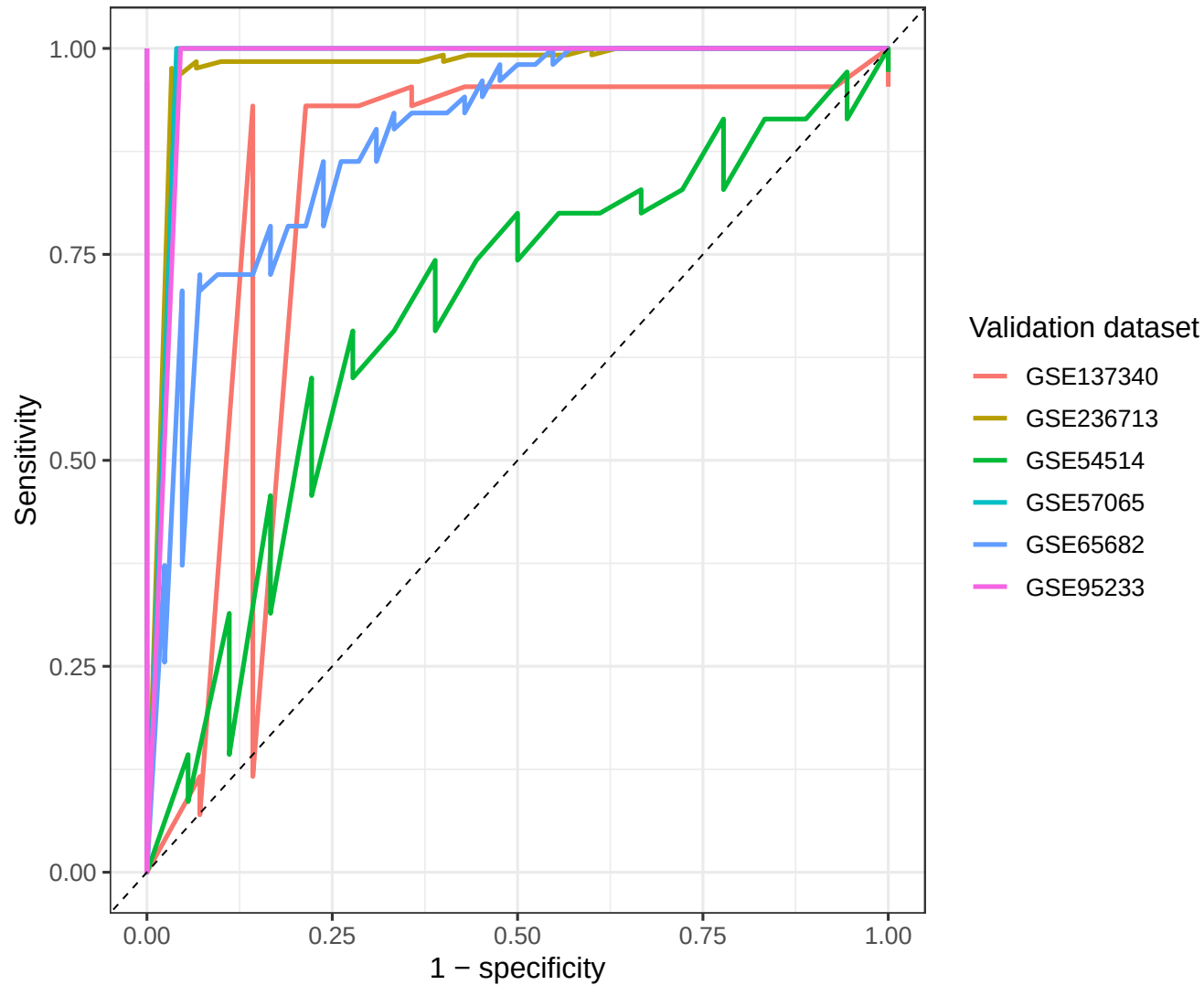
Leave-one-dataset-out ROC curves
