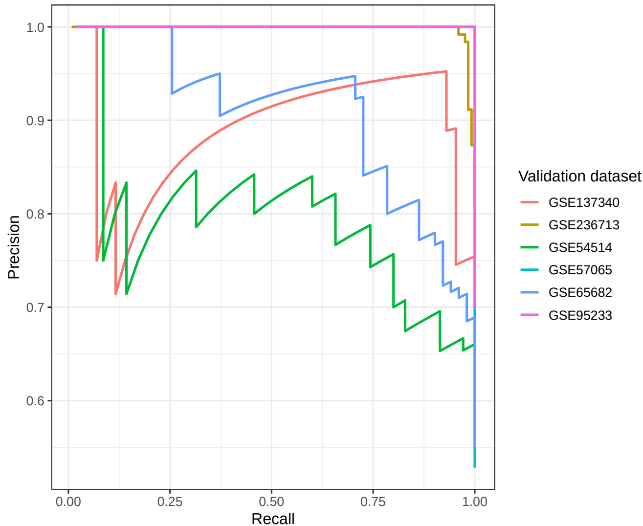
Leave-one-dataset-out precision-recall curves
