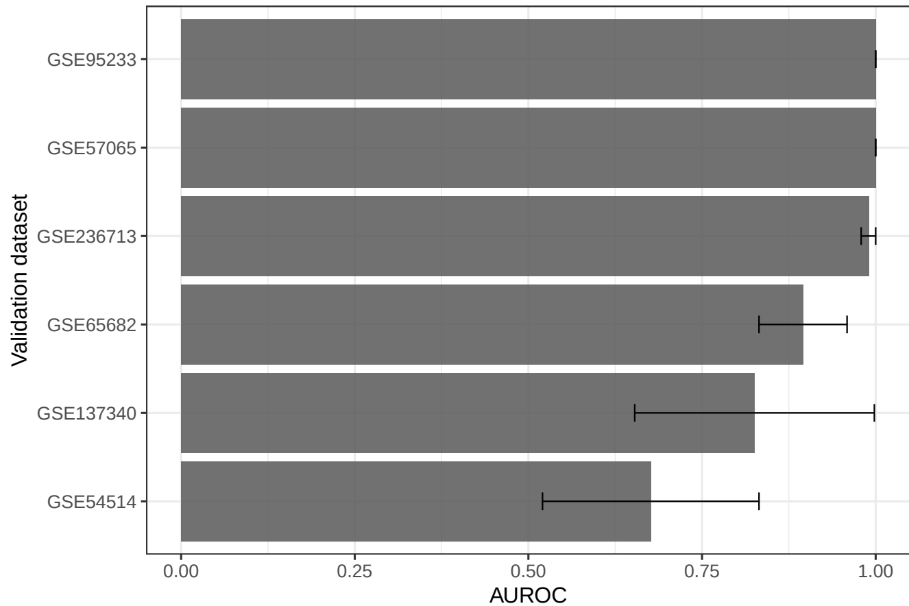
External validation AUROC by leave-one-dataset-out fold
